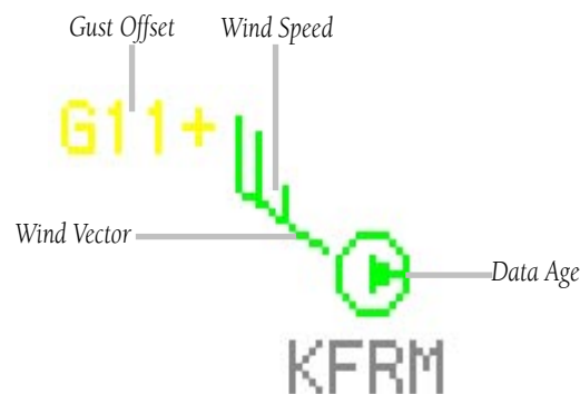
Figure 14-37 Wind Symbol
